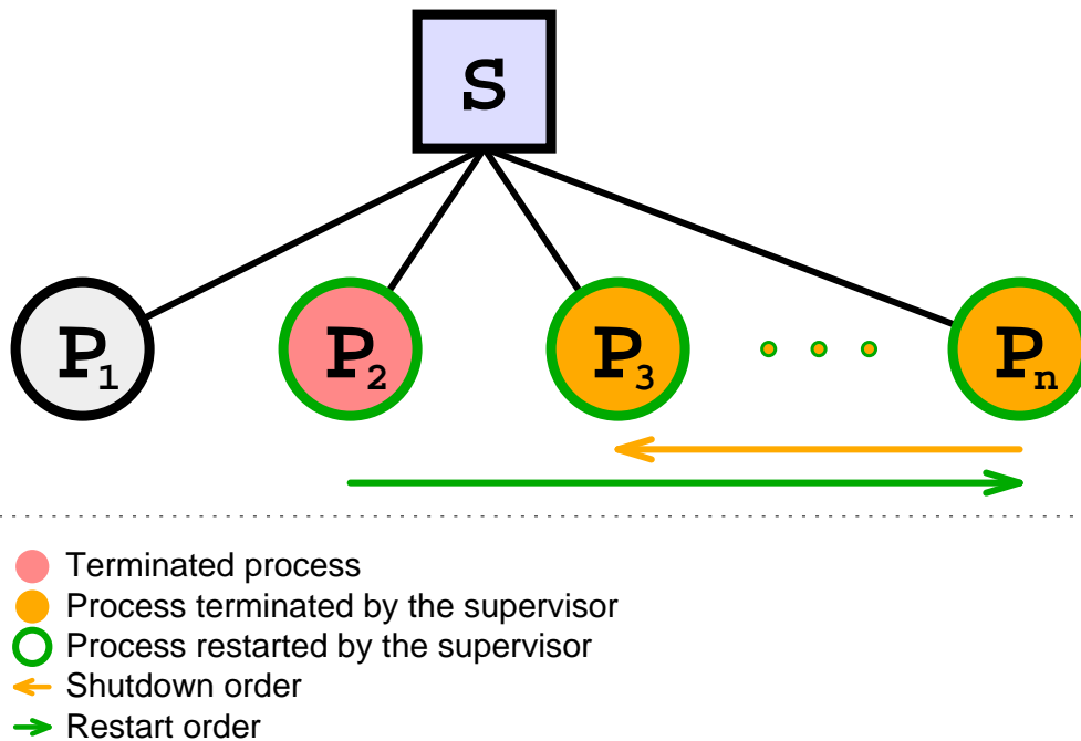
Figure 5.3: Rest_For_One Supervision
