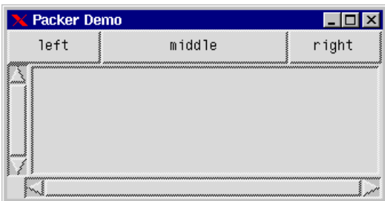
Figure 7.2: Resized Frame
